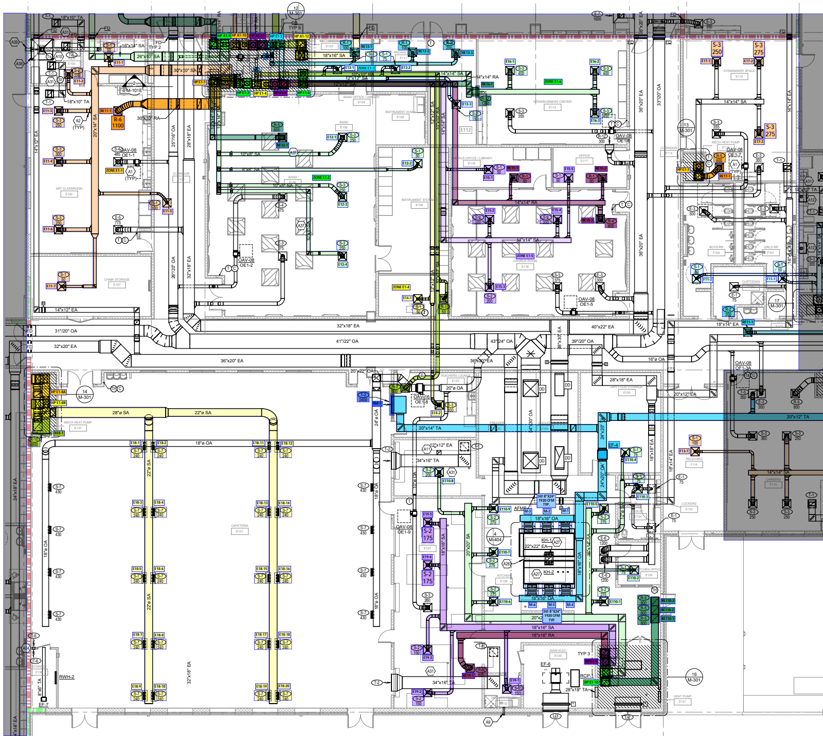
1 PARTIAL FIRST FLOOR PLAN - AIR DISTRIBUTION - AREA E
